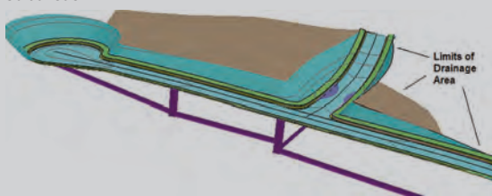
Precise gutter flow depths, spread and bypass calculations
